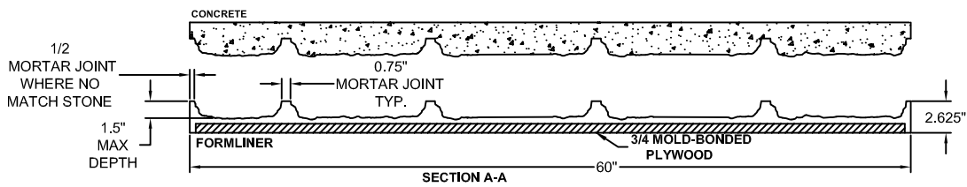
FORMLINER DETAIL
