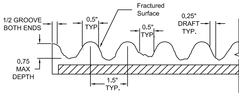
FORMLINER DETAIL
