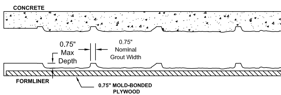
SECTION A-A FORMLINER DETAIL
