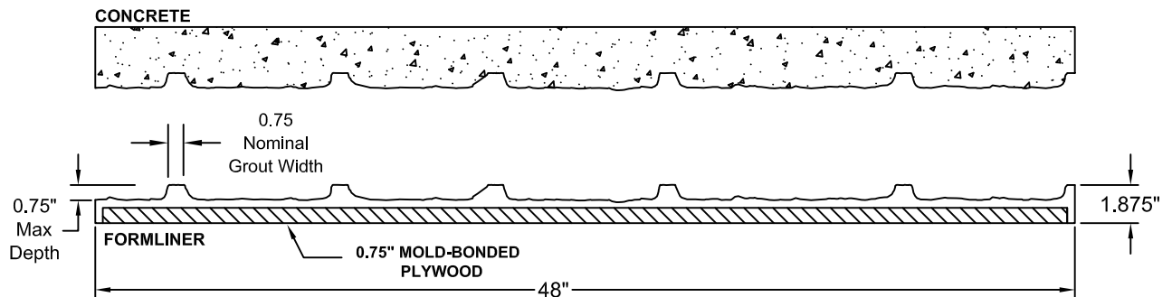
SECTION B-B FORMLINER DETAIL
