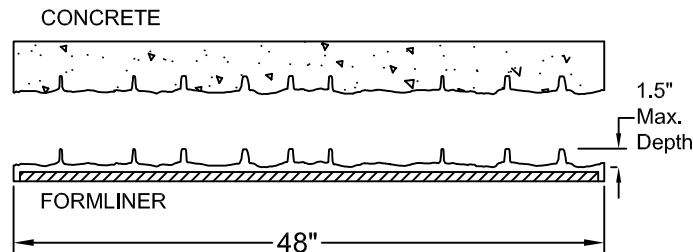
SECTION B-B
