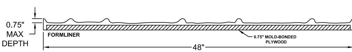
SECTION A-A FORMLINER DETAIL
