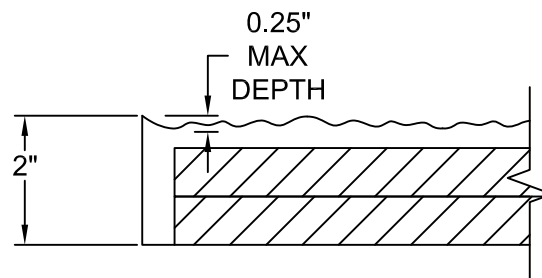
FORMLINER DETAIL
