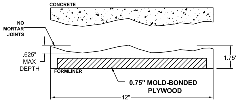
FORMLINER DETAIL
