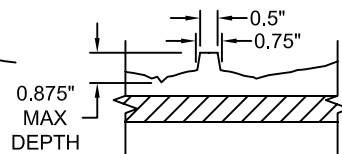
FORMLINER DETAIL
