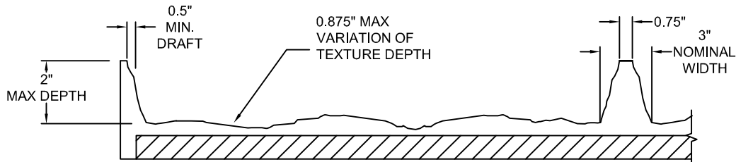
FORMLINER DETAIL
