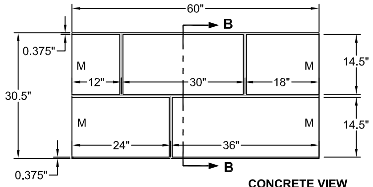
CONCRETE VIEW
