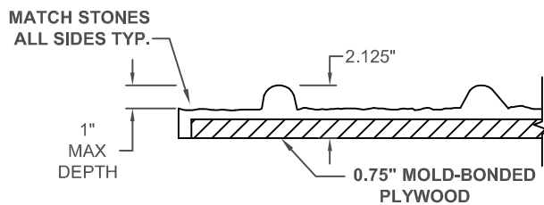
Formliner Detail
