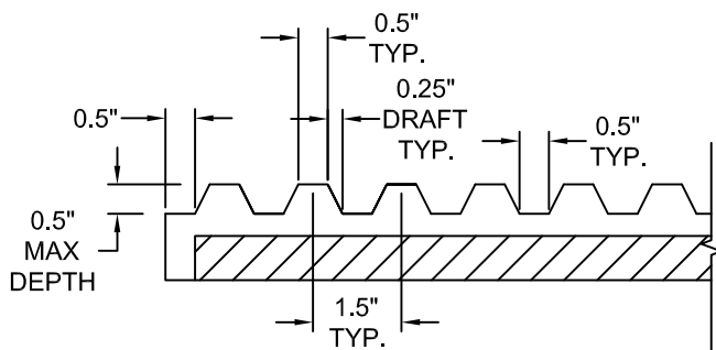
FORMLINER DETAIL
