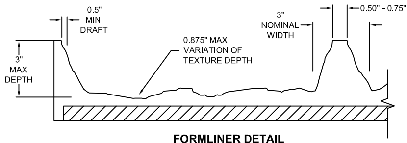
FORMLINER DETAIL
