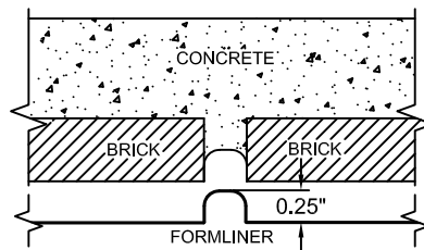
FORMLINER DETAIL
