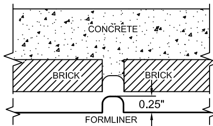
FORMLINER DETAIL
