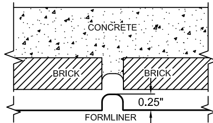
FORMLINER DETAIL
