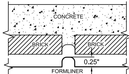
FORMLINER DETAIL
