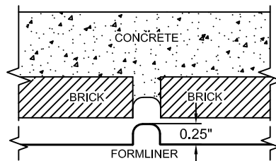
FORMLINER DETAIL
