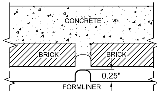
FORMLINER DETAIL
