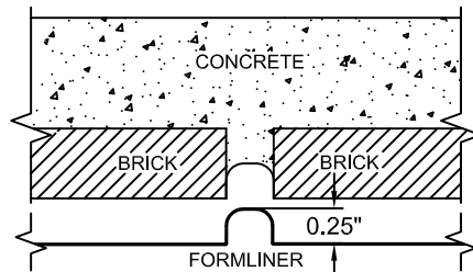
FORMLINER DETAIL
