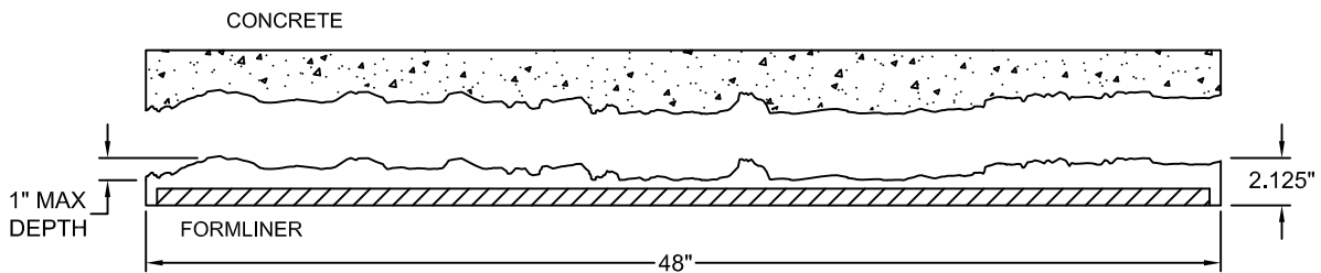
SECTION A-A FORMLINER DETAIL
