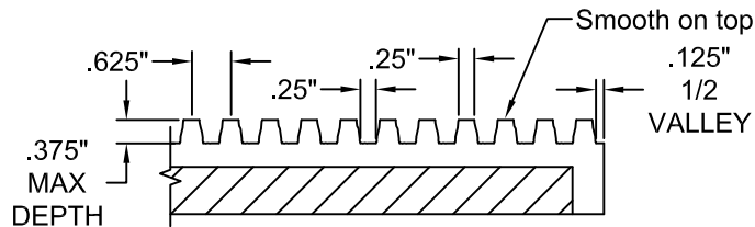
FORMLINER DETAIL
