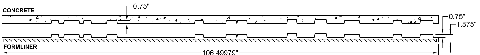
SECTION B-B
