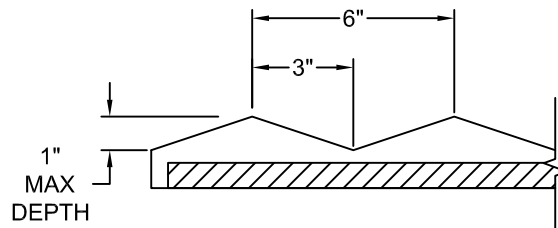
FORMLINER DETAIL
