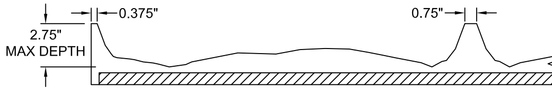
FORMLINER DETAIL
