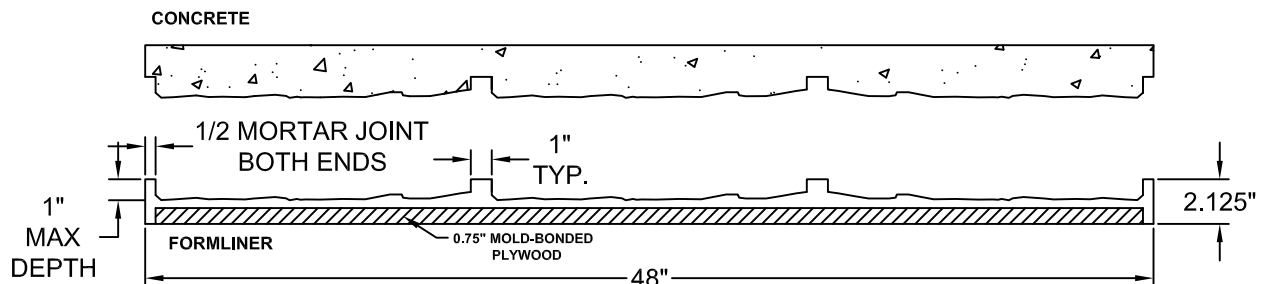
SECTION A-A FORMLINER DETAIL
