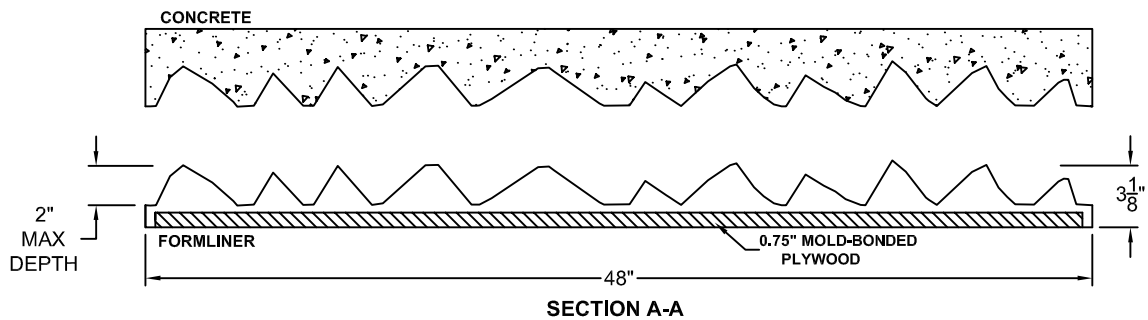
FORMLINER DETAIL
