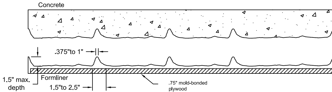
SECTION A-A FORMLINER DETAIL
