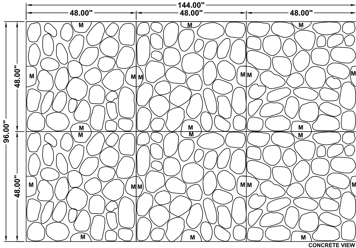
CONCRETE VIEW
