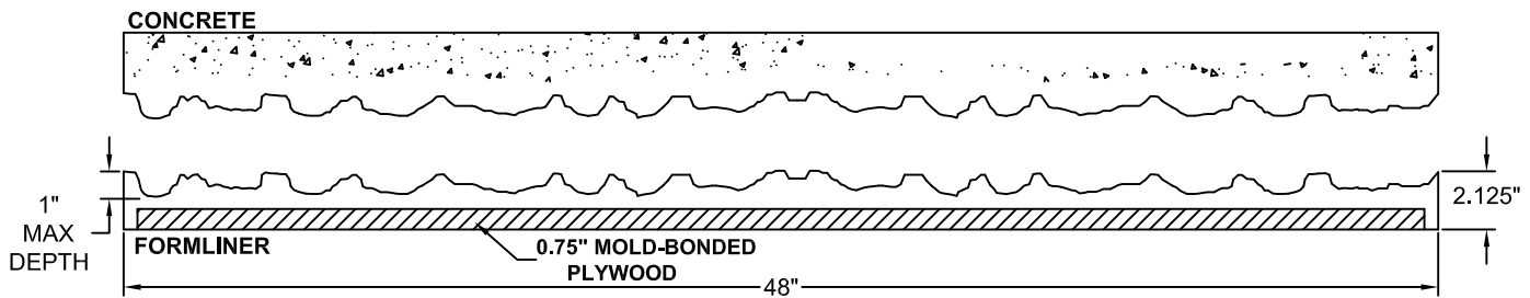
SECTION A-A FORMLINER DETAIL
