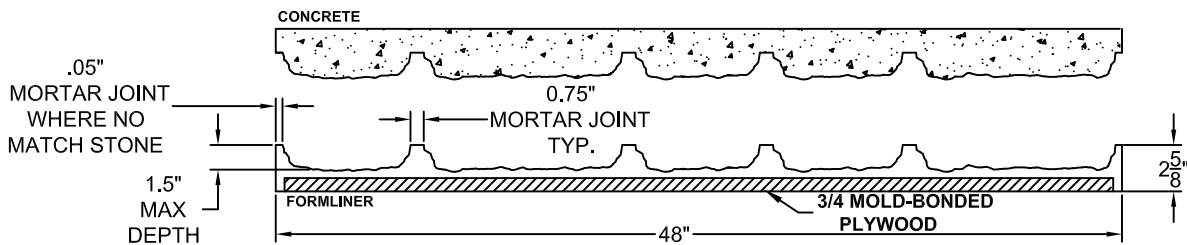
SECTION A-A FORMLINER DETAIL
