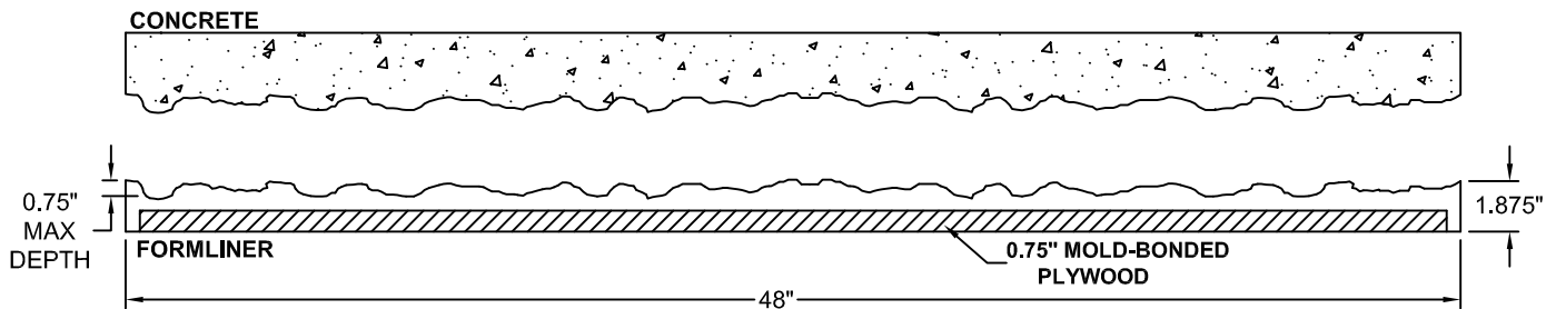
SECTION A-A FORMLINER DETAIL
