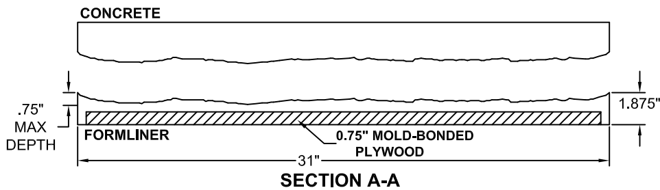
SECTION A-A FORMLINER DETAIL
