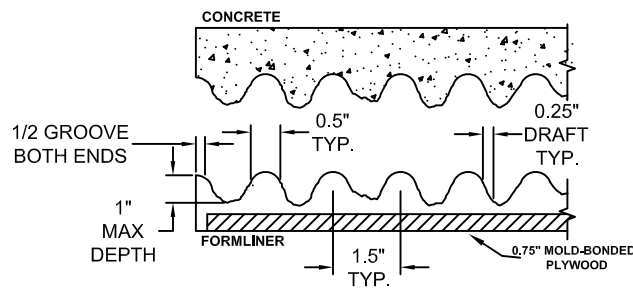
FORMLINER DETAIL
