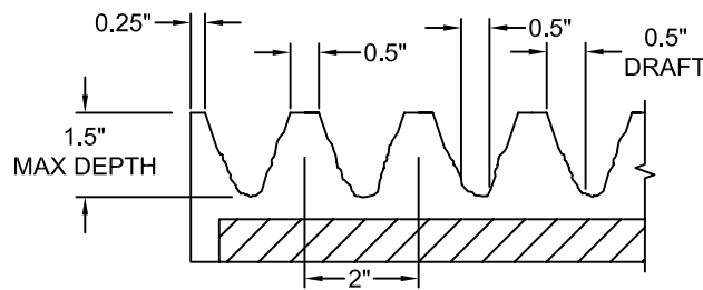
FORMLINER DETAIL
