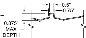
FORMLINER DETAIL
