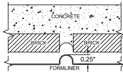
FORMLINER DETAIL
