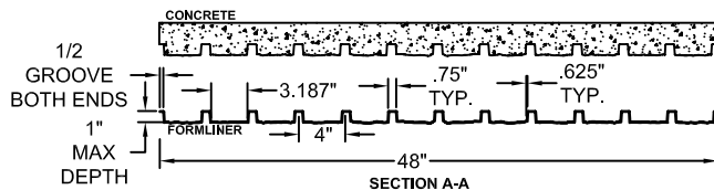
FORMLINER DETAIL
