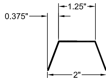
AT PANEL-TO-PANEL JOINT FORMLINER DETAIL
