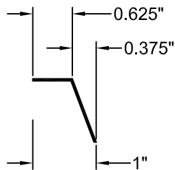
DETAIL OF PERIMETER REVEAL FORMLINER DETAIL
