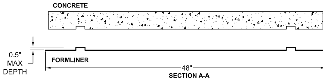
FORMLINER DETAIL
