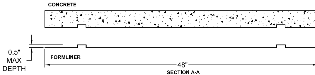
FORMLINER DETAIL
