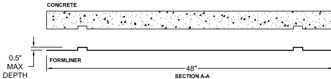
FORMLINER DETAIL
