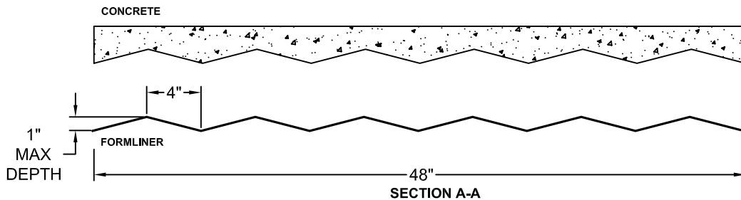
FORMLINER DETAIL
