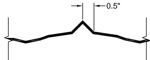
FORMLINER DETAIL - MIDDLE
