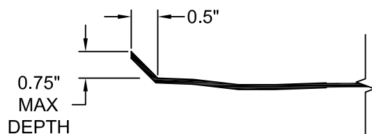
FORMLINER DETAIL - SIDES
