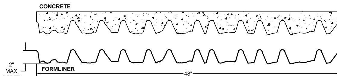
SECTION A-A FORMLINER DETAIL
