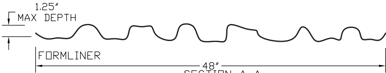
FORMLINER DETAIL
