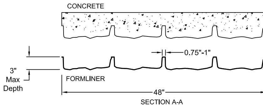
FORMLINER DETAIL
