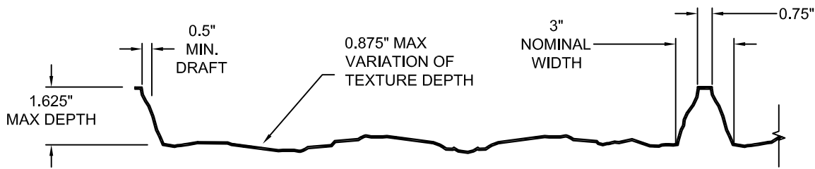
FORMLINER DETAIL
