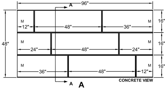
A (1.625" DEPTH)
