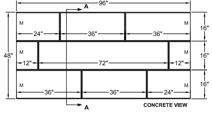
B (1.625" DEPTH)
