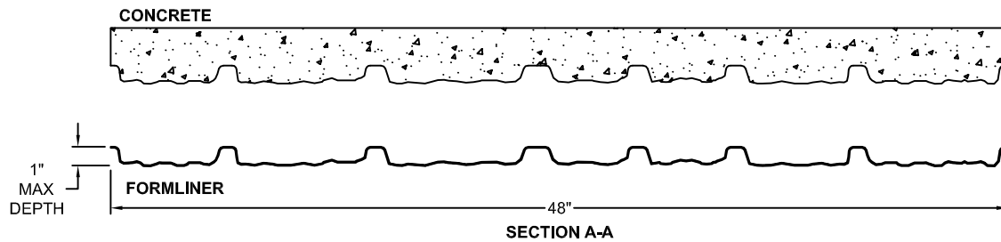
FORMLINER DETAIL
