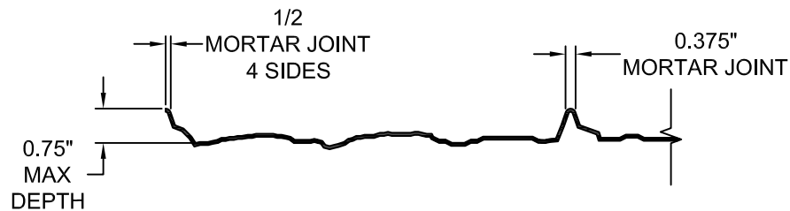
FORMLINER DETAIL
